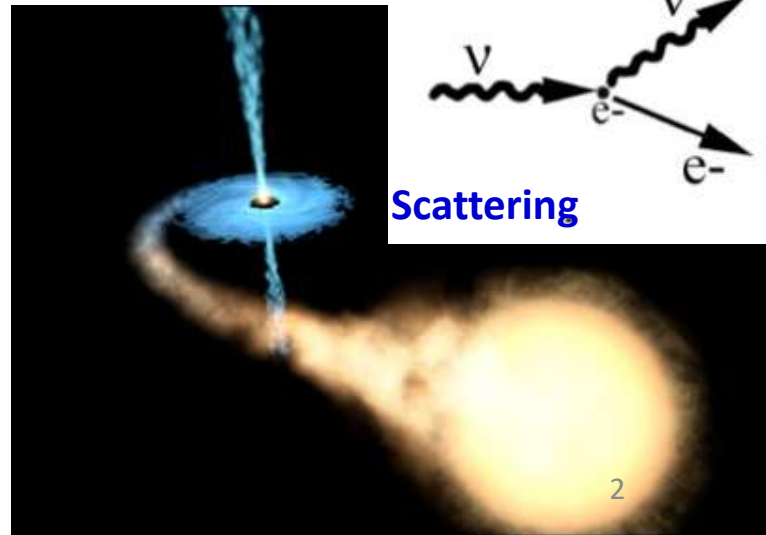
Cygnus X-1
