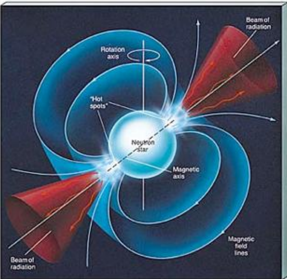
Synchrotron emission
