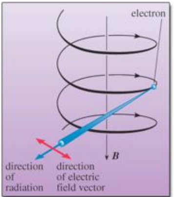
Synchrotron emission
