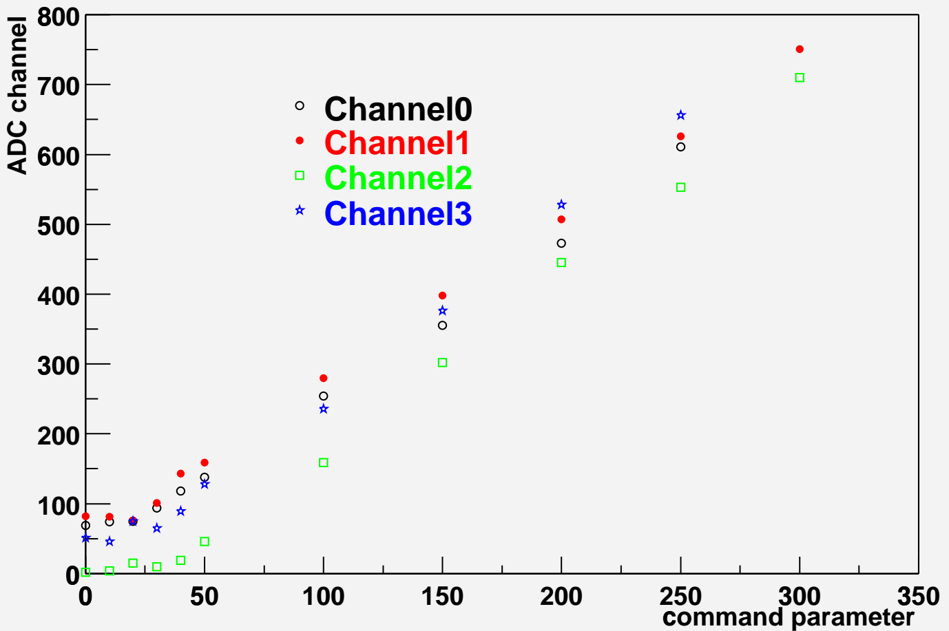
Command parameter vs. ADC channel of threshold level
